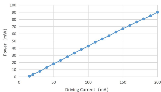
P-I Curve
