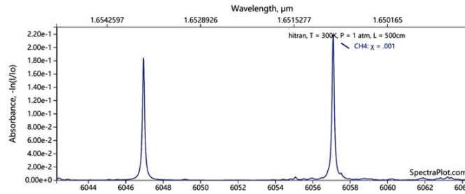
TDLAS: 1650.9nm 1653.7nm
