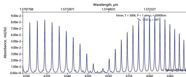
TDLAS: 1572/1578/1580nm
